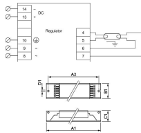
Specifications Philips HF-R 136 TL-D EII 220-240V for 1x36W
